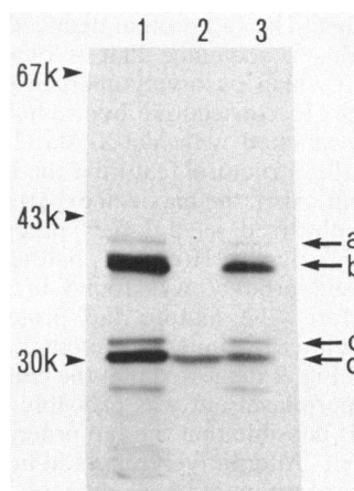
FIG. 4. Location of the Iap protein in the maxicells. Cells of CSR603 carrying pIN9054 labeled with [ 35 S]methionine were mixed with nonlabeled FE15 cells carrying the same plasmid and then treated by cold osmotic shock. After centrifugation at low speed, the supernatant and cell pellets obtained were treated by sodium dodecyl sulfate-polyacrylamide gel electrophoresis and fluorography. Lanes: 1, total cell fraction; 2, osmotic shock fluid; 3, cell fraction after osmotic shock treatment. a and b, iap gene product and its presumptive processed product, respectively; c and d, precursor of β-lactamase and β-lactamase, respectively.
